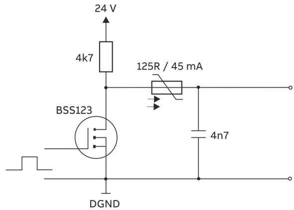
Figure 2: Digital output
