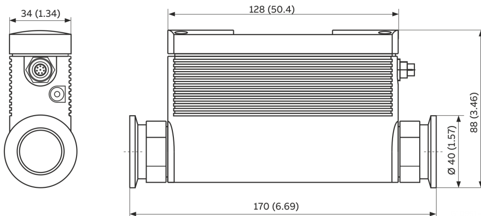
Figure 4: Flowmeter sensor FMT200-ECO2 with mounted small flange adapter
