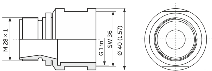
Figure 6: Dimensions in mm (in)
