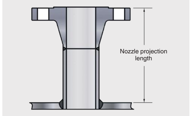
Nozzle projection
