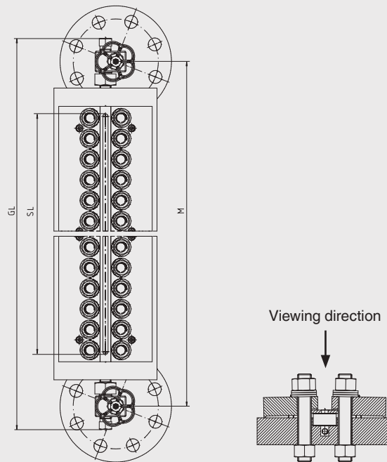
Version with valve head, top/bottom, model LGV-53
