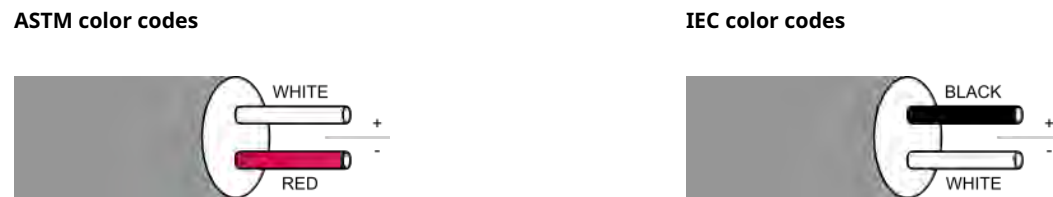
Figure 5: Type J Thermocouple Colors
