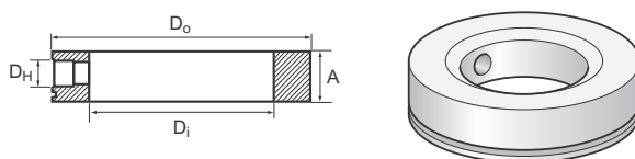
Figure 32: Flushing Connection Rings
