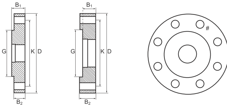
Figure 31: Proprietary Flanges
