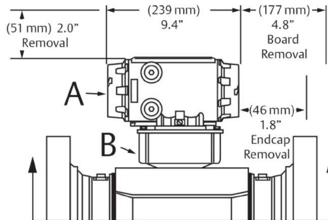
Figure 7: Optional installed position of enclosure housing (9)
