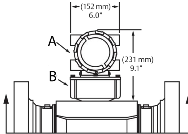
Figure 6: Standard installed position of enclosure housing (8)(9)
