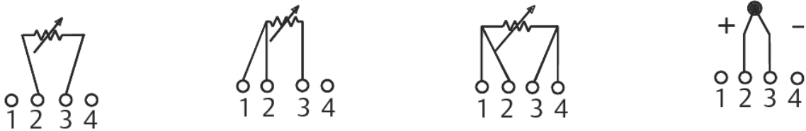
Figure 3: Rosemount 648 Wireless Sensor Connections
