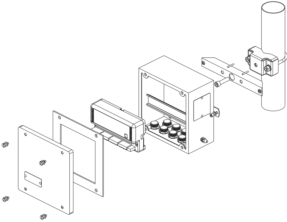
Figure 11: Mount stainless steel on vertical pipe
