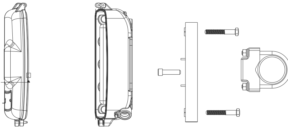
Figure 10: Mount aluminum on a vertical pipe
