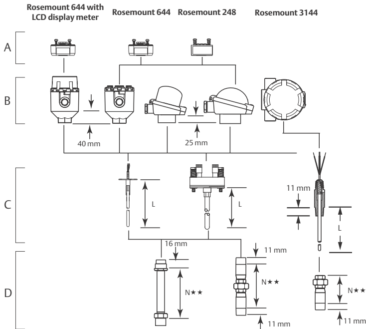
Figure 7: Sensor Assembly Without Thermowell
